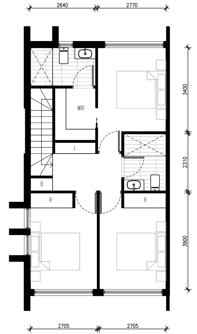
UPPER FLOOR
