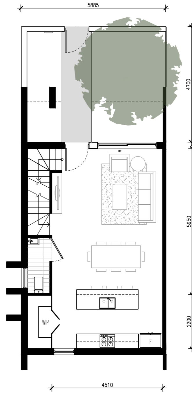
GROUND FLOOR
